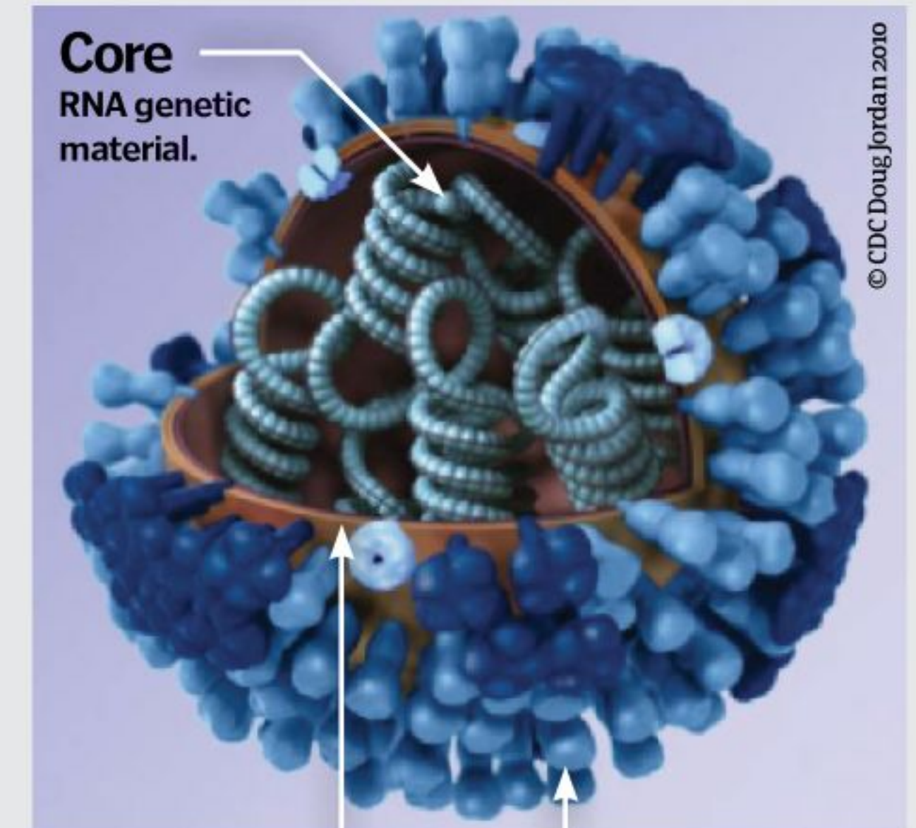
Capsid This protein coat encloses the virus's genetic information within the host cell.
